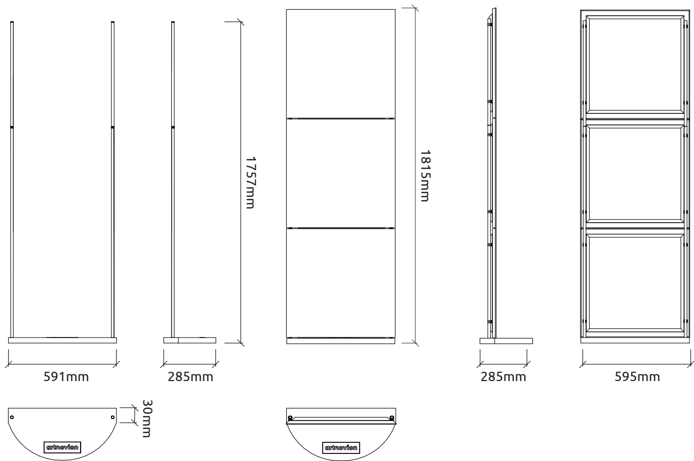
Mobile Wall | 595x1815x285mm
