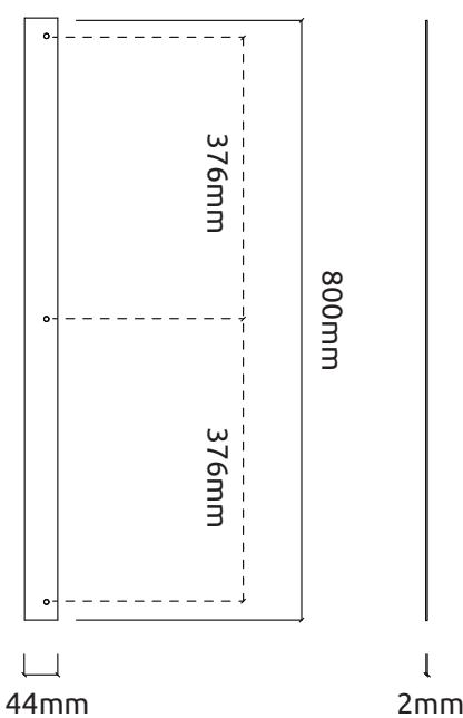
Panelling Metal Side Cover | 800x44x2mm
