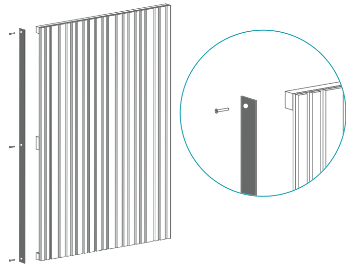
Vertical Mounting
