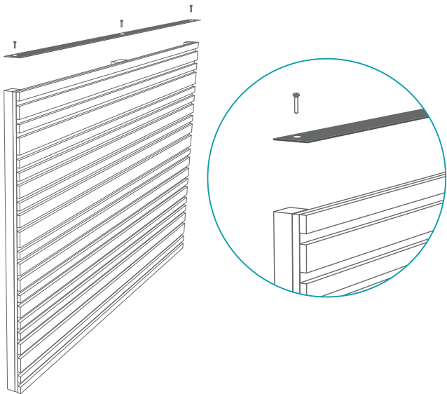
Horizontal Mounting
