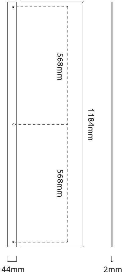
Panelling Metal Side Cover | 1184x44x2mm
